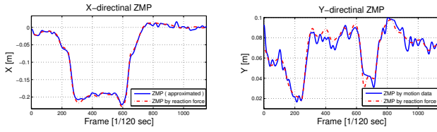
Fig. 2. Compare with ZMP trajectory calculated by reaction forces \mathbf{P} and achieved simplified human model \mathbf{P}^{appr} , for a simple whole-body motion
